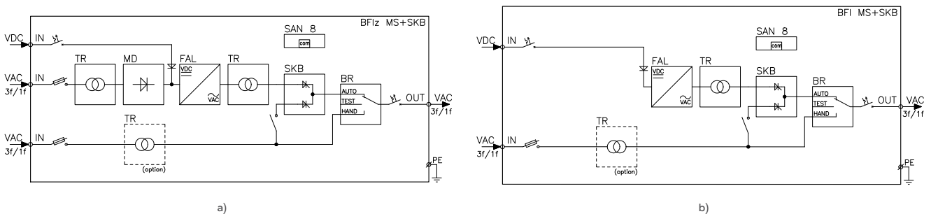
Fig. 61. Block diagram of the inverter cabinet in a free design: a) the BFIz type with the SKB bypass; b) the BFI type with the SKB bypass.
