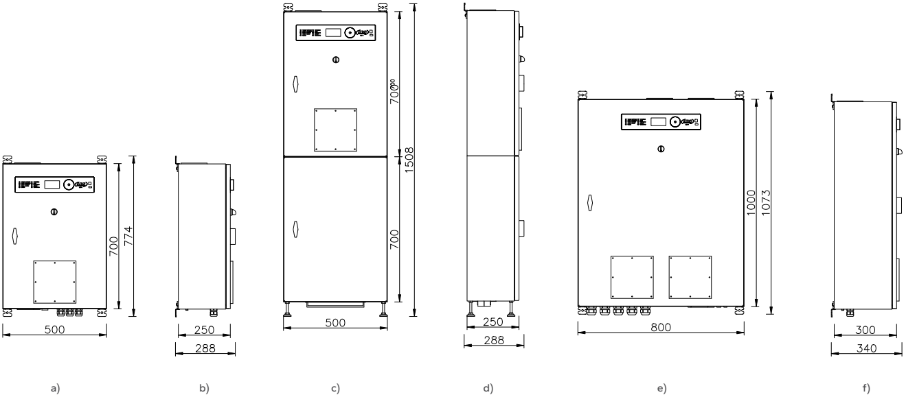
Fig. 76. Views with dimensions of the BFIpz / BFIp type inverter compact: a) CW6 compact – front view; b) CW6 compact – left-side view; c) CS6 compact – front view; d) CS6 compact – left-side view; e) CW1 compact – front view; f) CW1 compact – left-side view.
