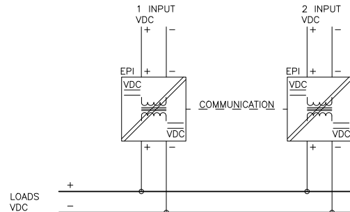
Fig. 26. DC/DC converter connection diagram – ATSE DC
