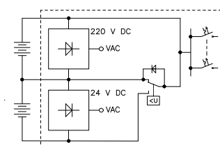
Fig. 6. A rectifier with an internal battery current measurement and the booster battery
