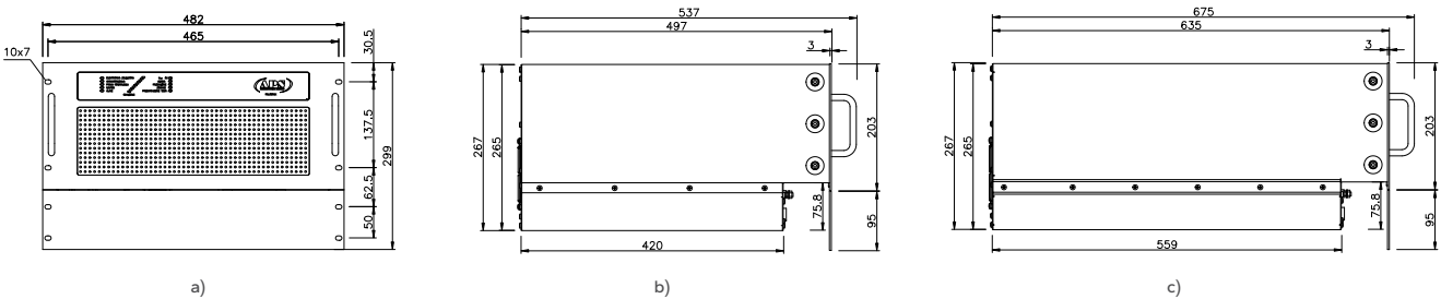
Fig. 94. Views with dimensions of the HPI type frequency converter module: a) front view in the M3 and M5 enclosure; b) left-side view in the M3 enclosure; c) left-side view in the M5 enclosure.
