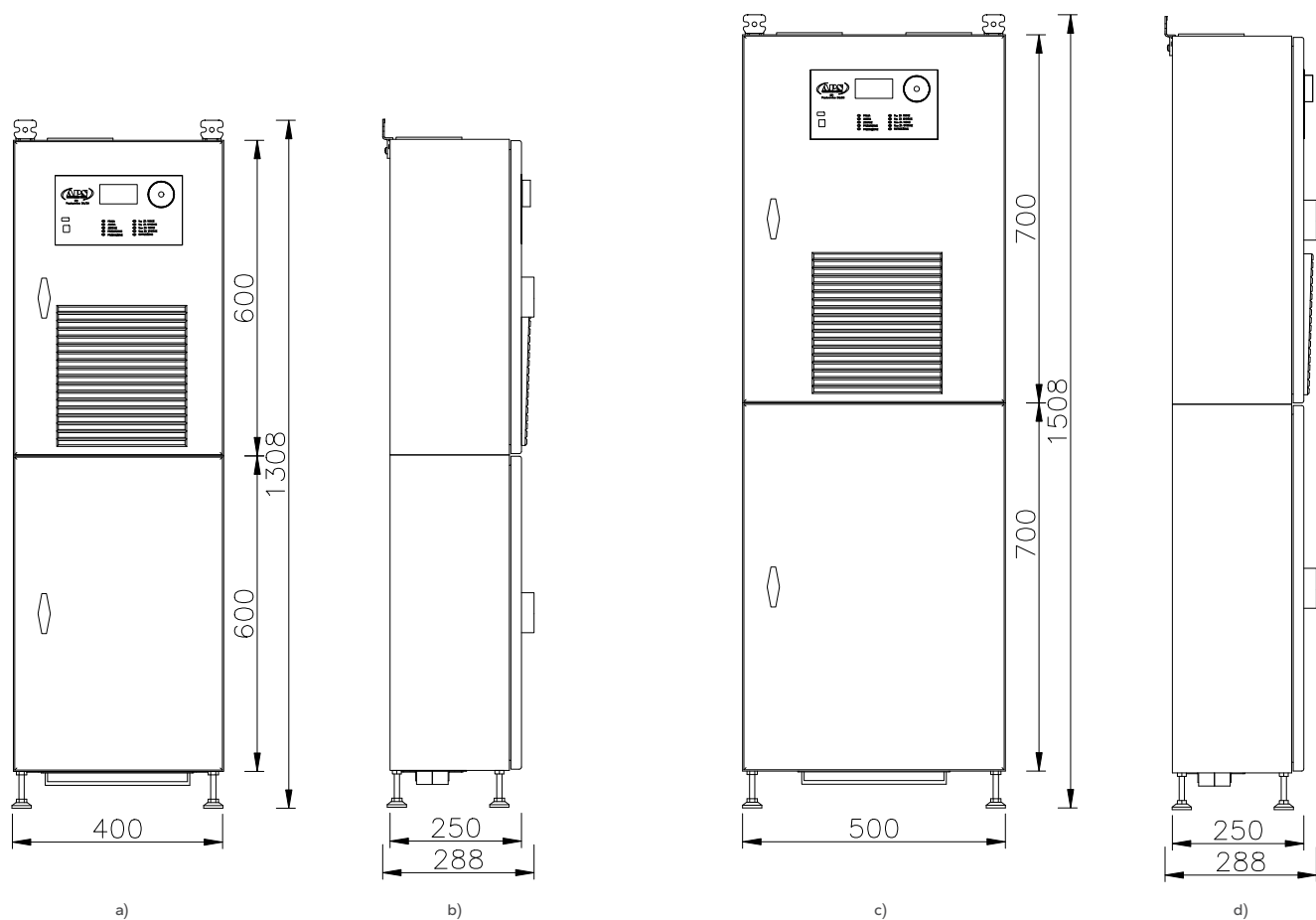
Fig. 40. Views with dimensions of the EPI type converter compact (standing enclosure): a) CS4 compact – front view; b) CS4 compact – left-side view; c) CS6 – front view; d) CS6 compact – left-side view.
