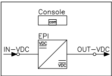
Fig. 22. General block diagram of the DC/DC converter system
