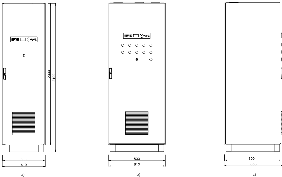
Fig. 97. Views with dimensions of the HPI type frequency converter cabinet:
