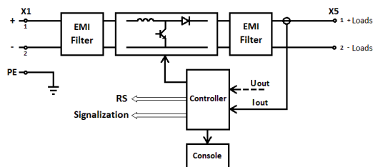
Fig. 24. Conceptual diagram of the converter without the EPIs type galvanic insulation
