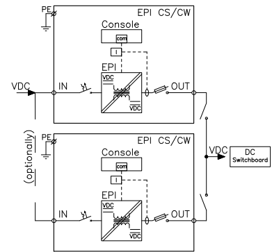
Fig. 39. Block diagram of the EPI type converter compact for parallel operation.
