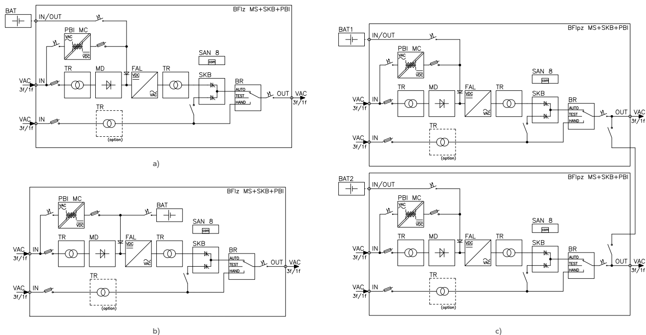
Fig. 87. Block diagram of the UPS system cabinet:
