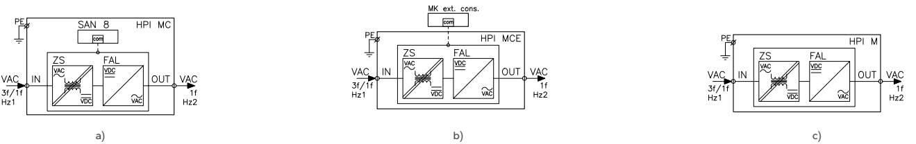
Fig. 93. Block diagram of the HPI type frequency converter module: a) with a built-in console; b) with an external MK console; c) without a console.
