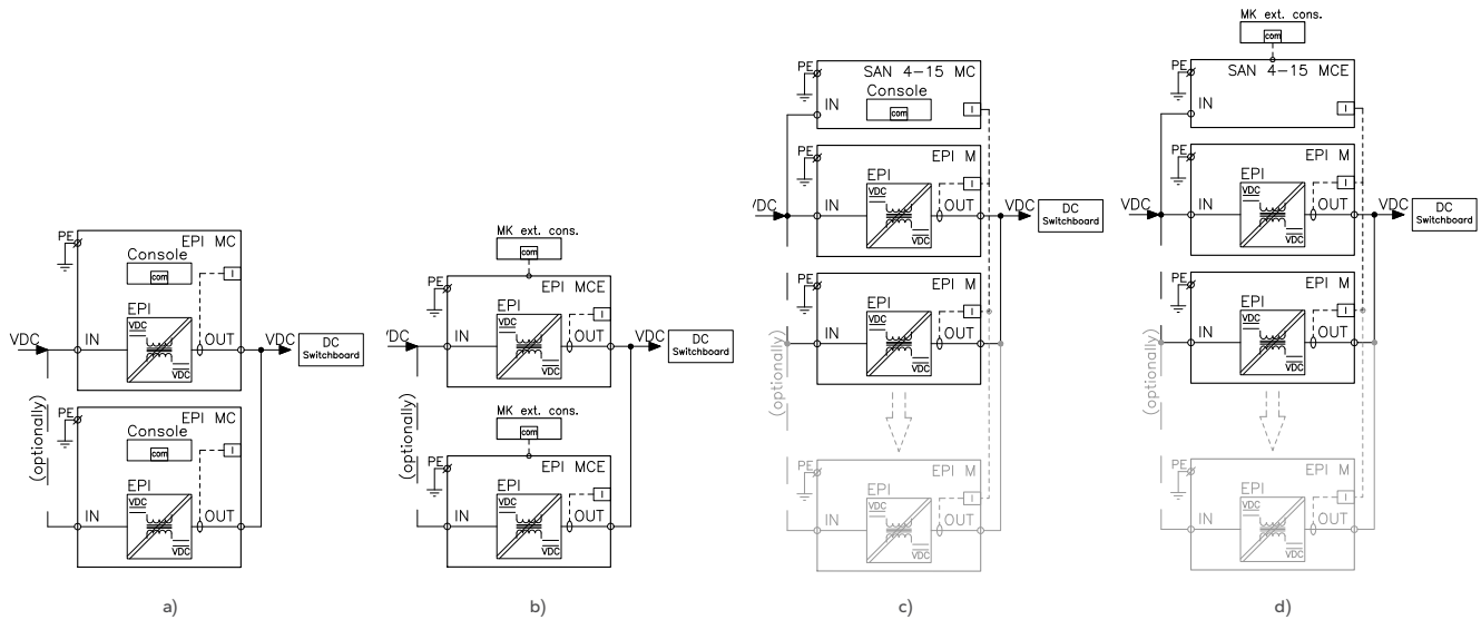
Fig. 29. Block diagram of the converter modules with the EPI type galvanic insulation for parallel operation: a) the EPI MC type modules system; b) the EPI MCE type modules system with an external MK console; c) the EPI M type modules and the SAN 4-15 MC type controller system; d) the EPI M type modules and the SAN 4-15 MCE type controller system with an external MK console.
