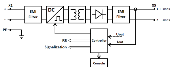
Fig. 23. Conceptual diagram of the converter with the EPI type galvanic insulation
