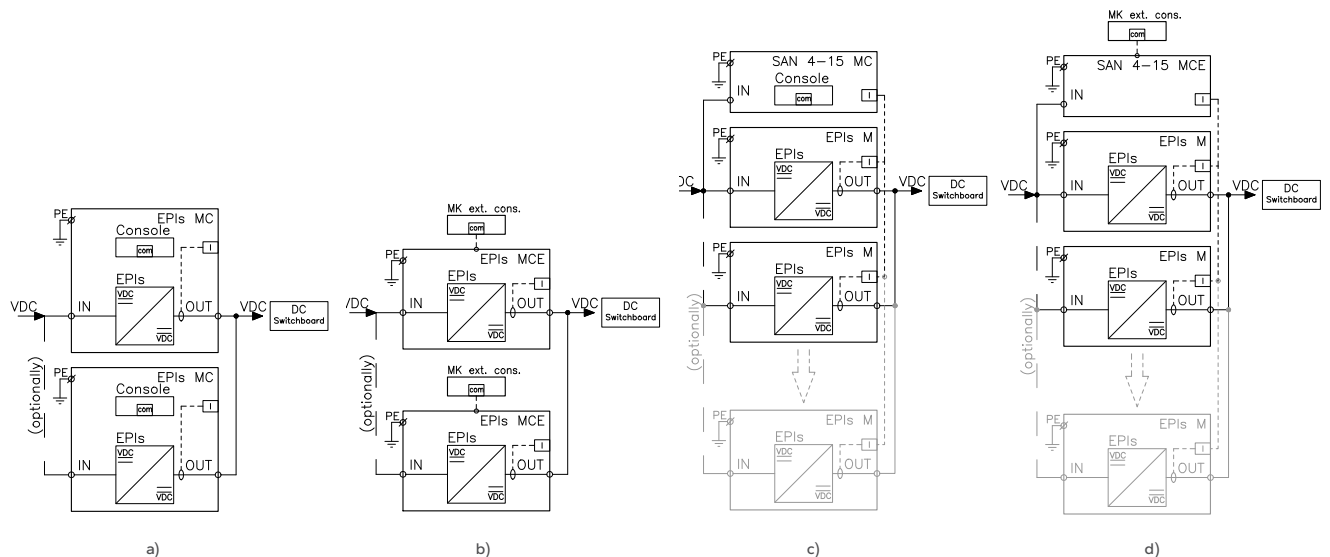
Fig. 30. Block diagram of the converter modules without the EPIs type insulation for parallel operation: a) the EPIs MC type modules system; b) the EPIs MCE type modules system with an external MK console; c) the EPIs M type modules and the SAN 4-15 MC type controller system; d) the EPIs M type modules and the SAN 4-15 MCE type controller system with an external MK console.
