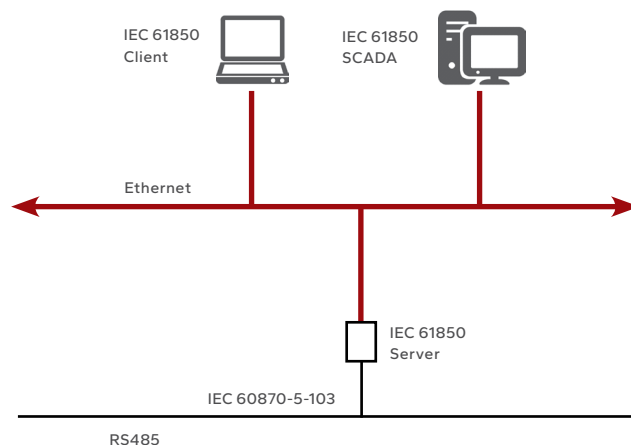
View of an example automatics system configuration according to IEC 61850
