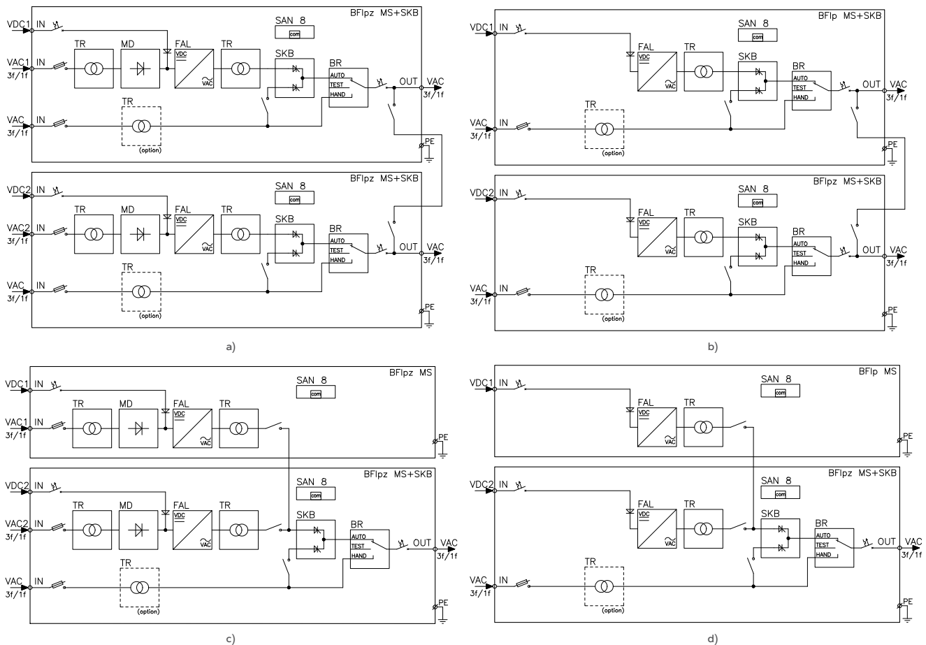
Fig. 67. Block diagram of the BFlpz / BFip type inverter cabinets in a free design for parallel operation with the SKB type bypass. Possible configurations:
