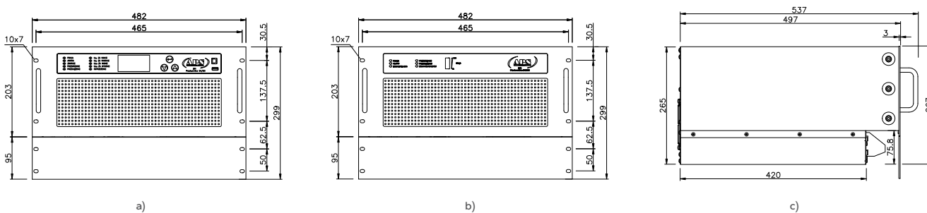
Fig. 32. Views with dimensions of the EPI M / MC / MCE type converter module in the M3 enclosure: a) front view – a module with a built-in console; b) front view – a module without a console; c) left-side view.
