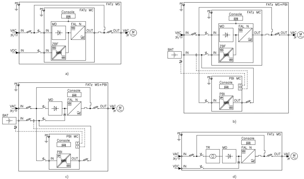
Fig. 104. Block diagram of the asynchronous motors power supply systems:
