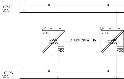
Fig. 25. DC/DC converter connection diagram – a redundant system
