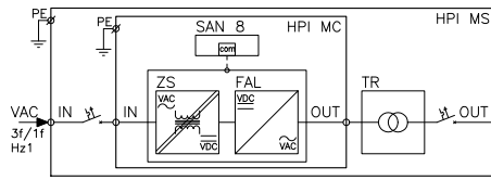
Fig. 95. Block diagram of the HPI type frequency converter cabinet in a modular design.
