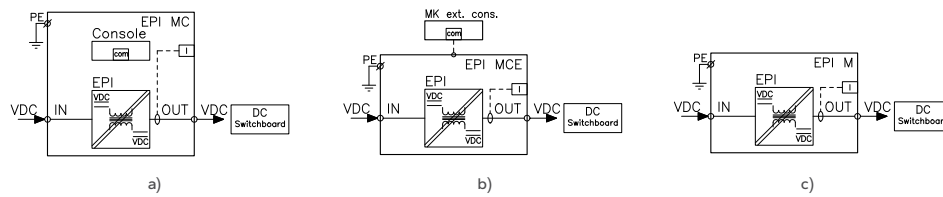
Fig. 27. Block diagram of the converter module with the EPI type galvanic insulation for autonomous operation: a) with a built-in console; b) with an external MK console; c) without a console.
