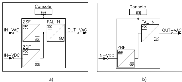
Fig. 100. General block diagram of the asynchronous motor power supply system: a) with the FATz type power supply unit; b) without the FAT type power supply unit.
