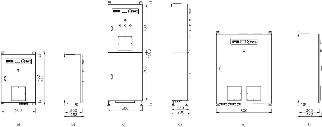
Fig. 99. Views with dimensions of the HPI type frequency converter compact: a) CW6 compact – front view; b) CW6 compact – left-side view; c) CS6 compact – front view; d) CS6 compact – left-side view; e) CW1 compact – front view; f) CW1 compact – left-side view.
