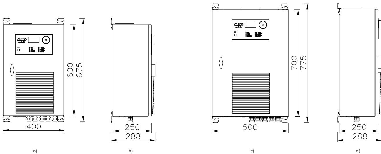
Fig. 41. Views with dimensions of the EPI type converter compact (wall-mounted enclosure): a) CW4 compact – front view; b) CW4 compact – left-side view; c) CW6 – front view; d) CW6 compact – left-side view.
