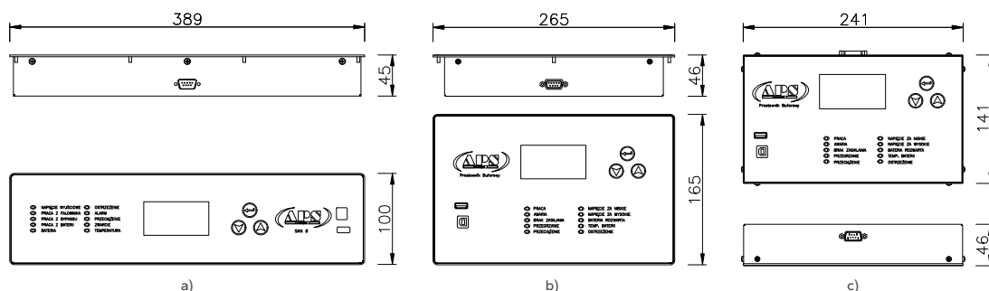
Fig. 106. Views of the MK type portable consoles: a) K1 console; b) K2 console; c) K3 console.
