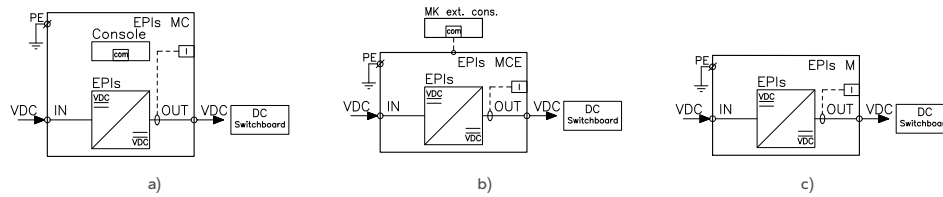
Fig. 28. Block diagram of the converter module without the EPIs type insulation for autonomous operation: a) with a built-in console; b) with an external MK console; c) without a console.
