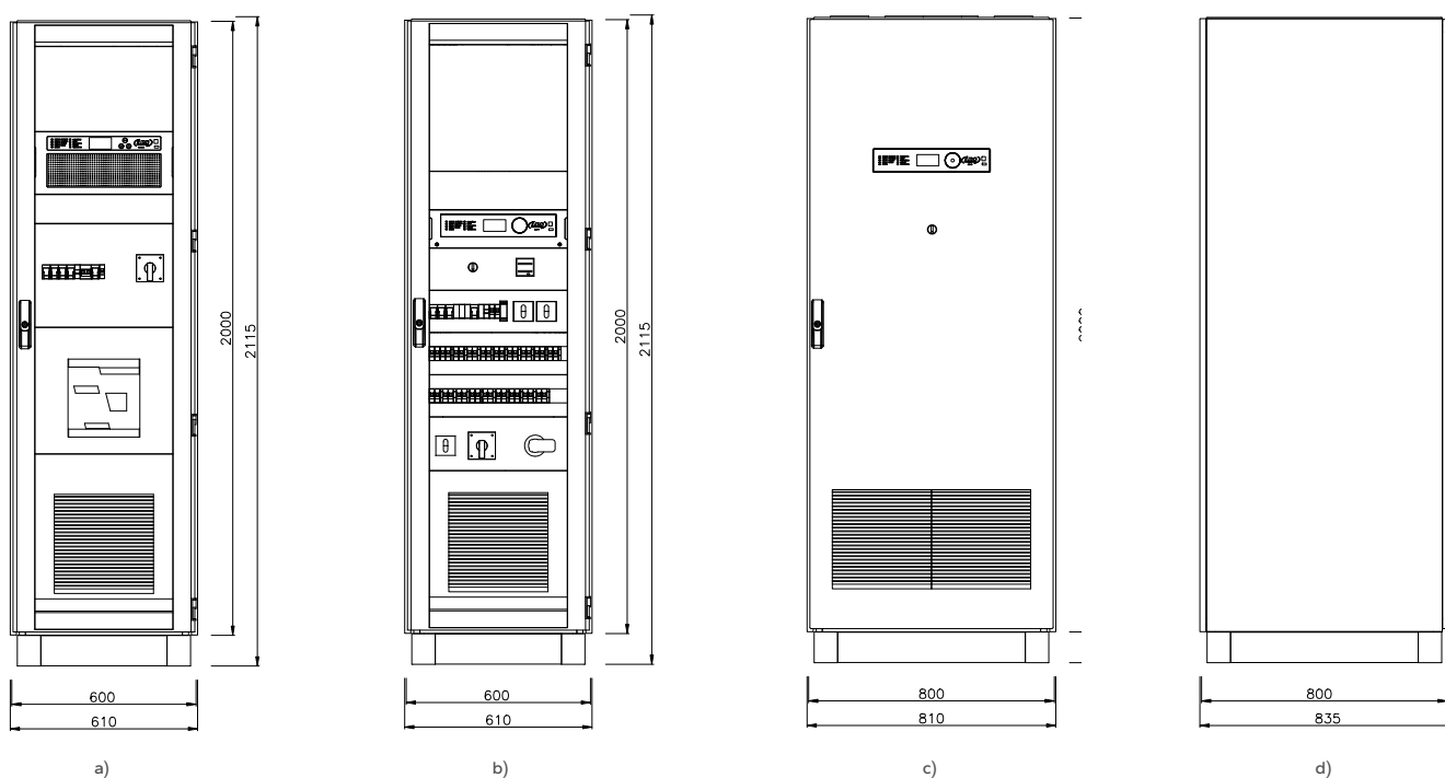
Fig. 62. Views with dimensions of the BFIZ / BFI type inverter cabinet:
