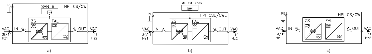
Fig. 98. Block diagram of the HPI type frequency converter compact: a) with a built-in console; b) with an external MK console; c) without a console.
