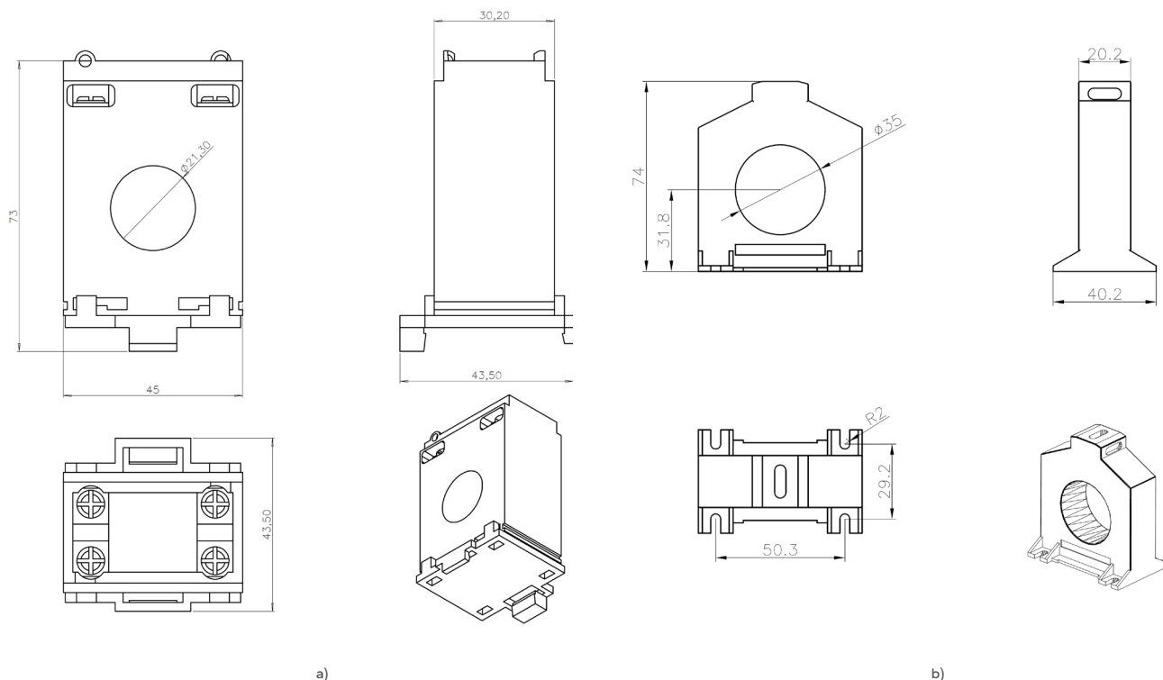
Fig. 107. Views with dimensions of the current transformers:
