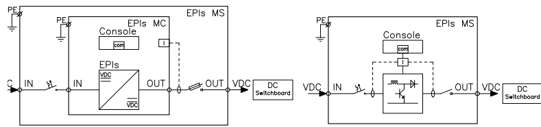
Fig. 34. Block diagram of the EPIs type converter cabinet for autonomous operation: a) modular design; b) free design.
