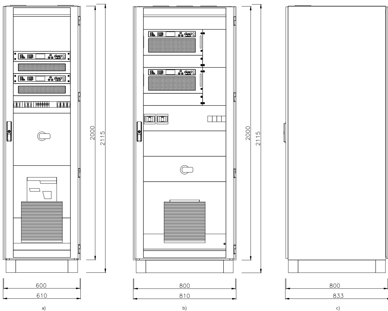
Fig. 37. Views with dimensions of the EPI / EPIs converter cabinet:
