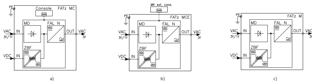
Fig. 101. Block diagram of the FAT type drive inverter module with a power supply unit: a) with a built-in console; b) with an external MK console; c) without a console.
