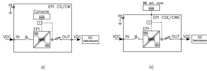
Fig. 38. Block diagram of the EPI type converter compact for autonomous operation: a) with a built-in console; b) with an external MK console.
