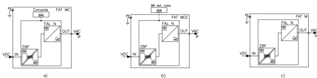
Fig. 102. Block diagram of the FATz type drive inverter module with a power supply unit: a) with a built-in console; b) with an external MK console; c) without a console.
