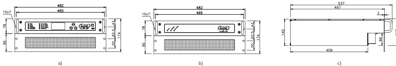
Fig. 31. Views with dimensions of the EPI M / MC / MCE type converter module in the M4 enclosure: a) front view – a module with a built-in console; b) front view – a module without a console; c) left-side view.
