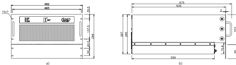
Fig. 103. Views with dimensions of the FATz / FAT MC type drive inverter: a) front view in the M5 enclosure; b) left-side view in the M5 enclosure.
