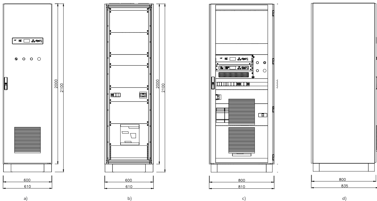
Fig. 105. Views with dimensions of the FATz / FAT type asynchronous motors power supply system cabinet: a) 600×800×2,000 cabinet – front view, closed door; b) 600×800×2,000 cabinet – front view, open door; c) 800×800×2,000 cabinet – front view; d) a cabinet of the depth of 800 mm – left-side view.
