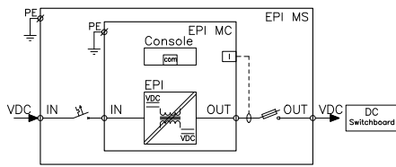
Fig. 33. Block diagram of the EPI type converter cabinet for autonomous operation
